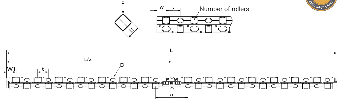
Snap-on cage
