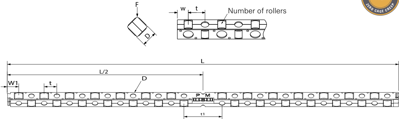
Snap-on cage
