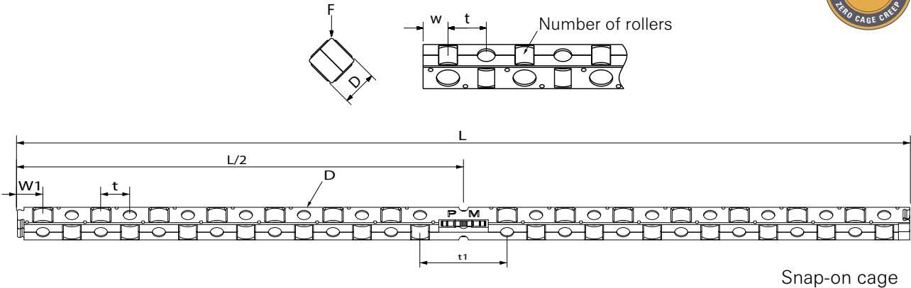
Snap-on cage
